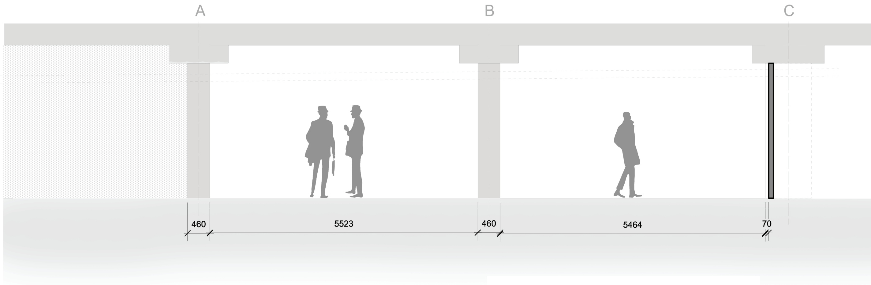
Space I - Section 'AA'
